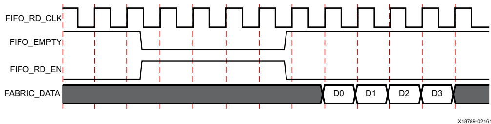
Figure 4-5: Bitslip Enabled and FIFO Read Enable User Controlled
