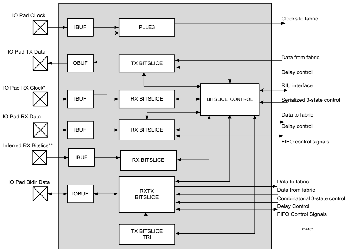
Figure 2-1: Representative Design
