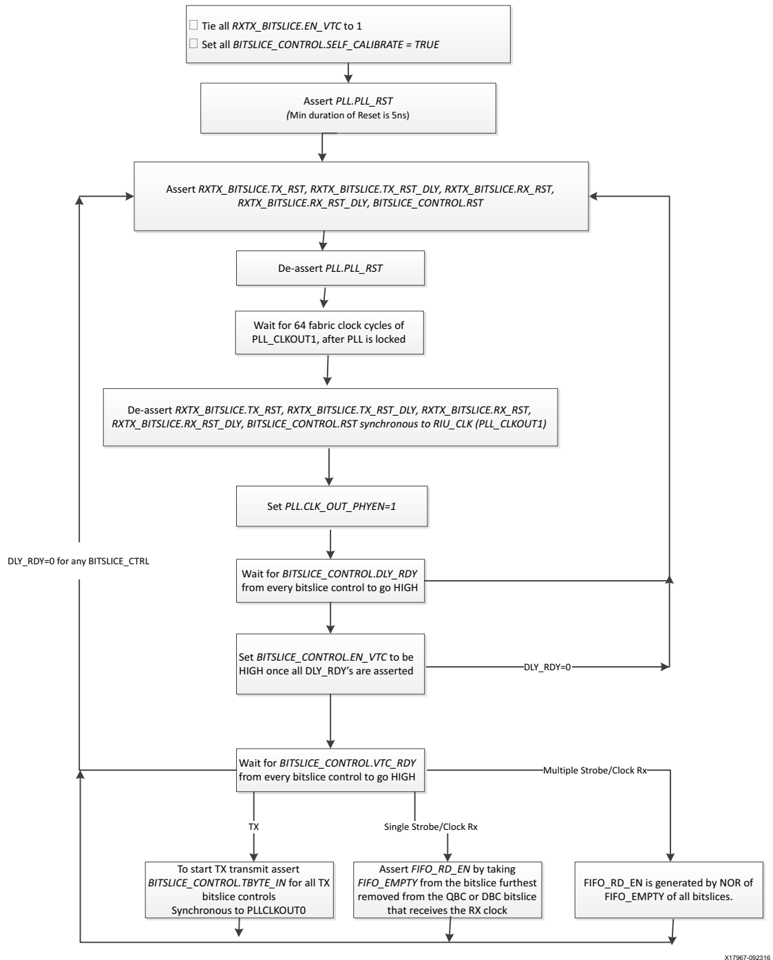
Figure 3-8: RIU From PLL
