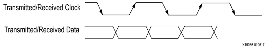
Figure 3-3: Center DDR
