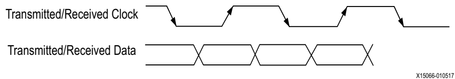
Figure 3-5: Center DDR Strobe
