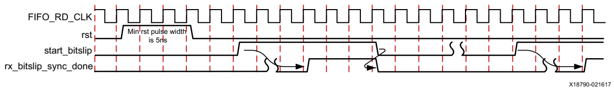
Figure 4-4: Bitslip Disabled and FIFO Read Enable User Controlled
